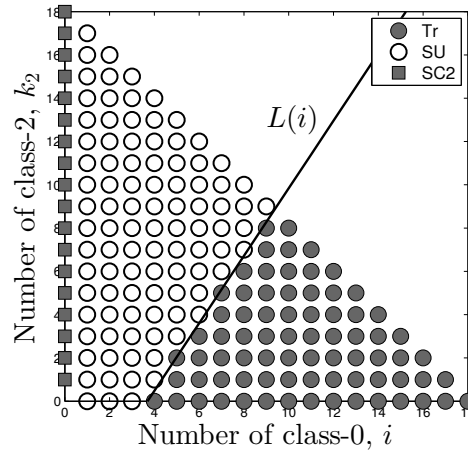
Figure 1 Visual description of the optimal policy when k_1 = 0 and
