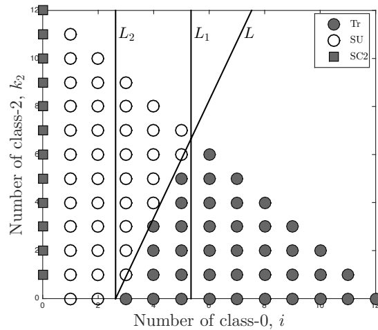
Figure 2 Visual description of the three heuristic policies
